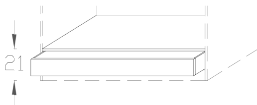
Predal 2 delni L= 97,5cm
